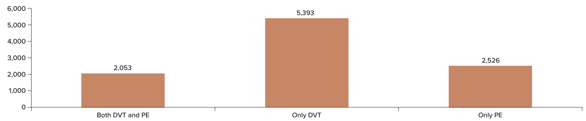
Figure 3. Low-Molecular-Weight Heparins
