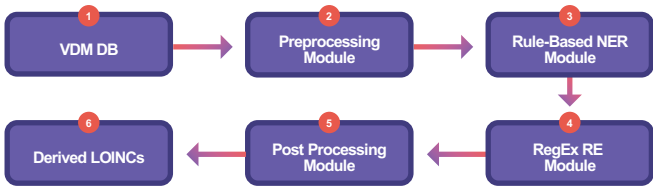
Figure 3 | Rule-Based NLP Process Flow Diagram
