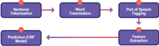
Figure 2 | Steps in CRF NER Module
