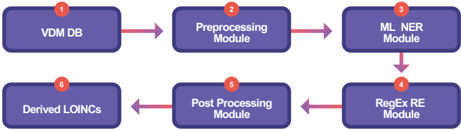
Figure 4 | ML-Based NLP Process Flow Diagram
