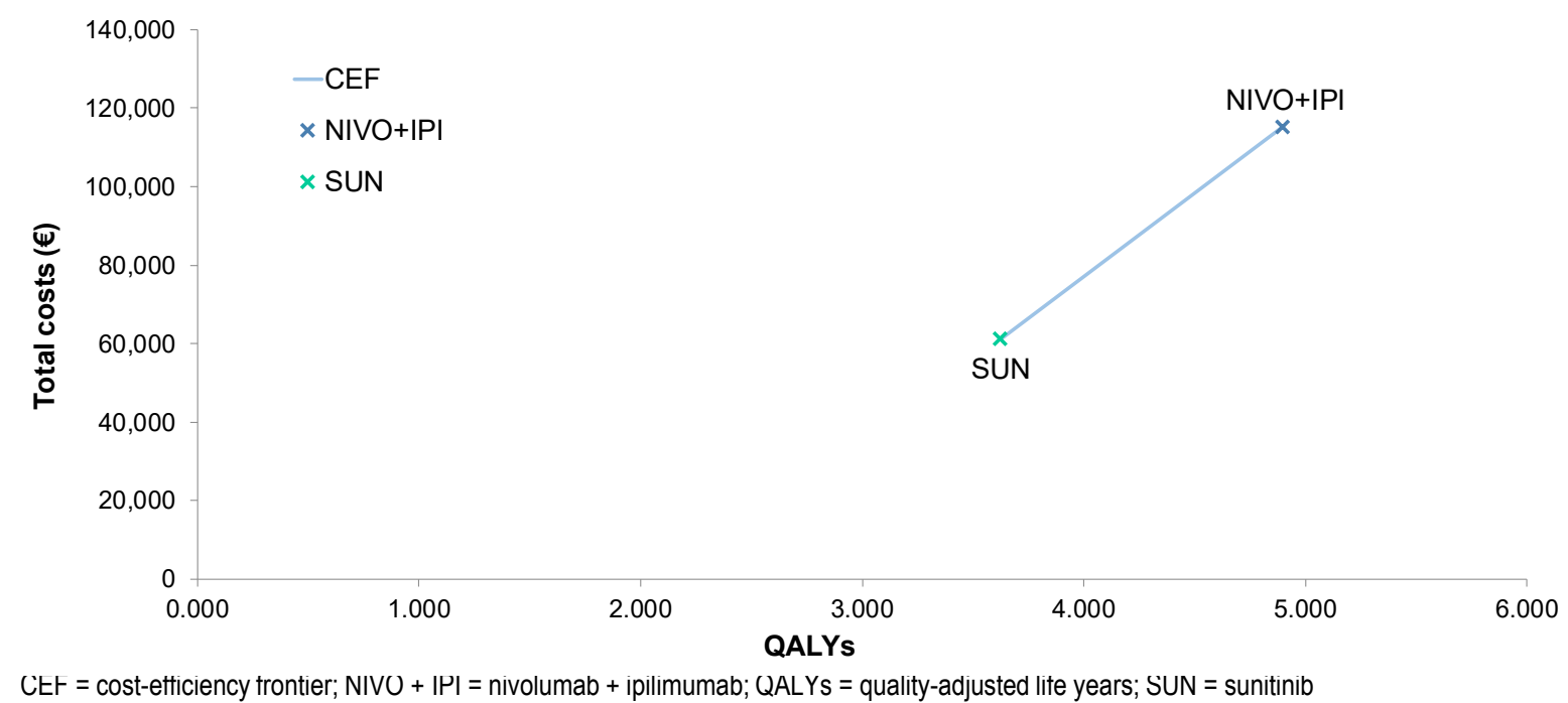
Figure 3. Efficiency frontier
