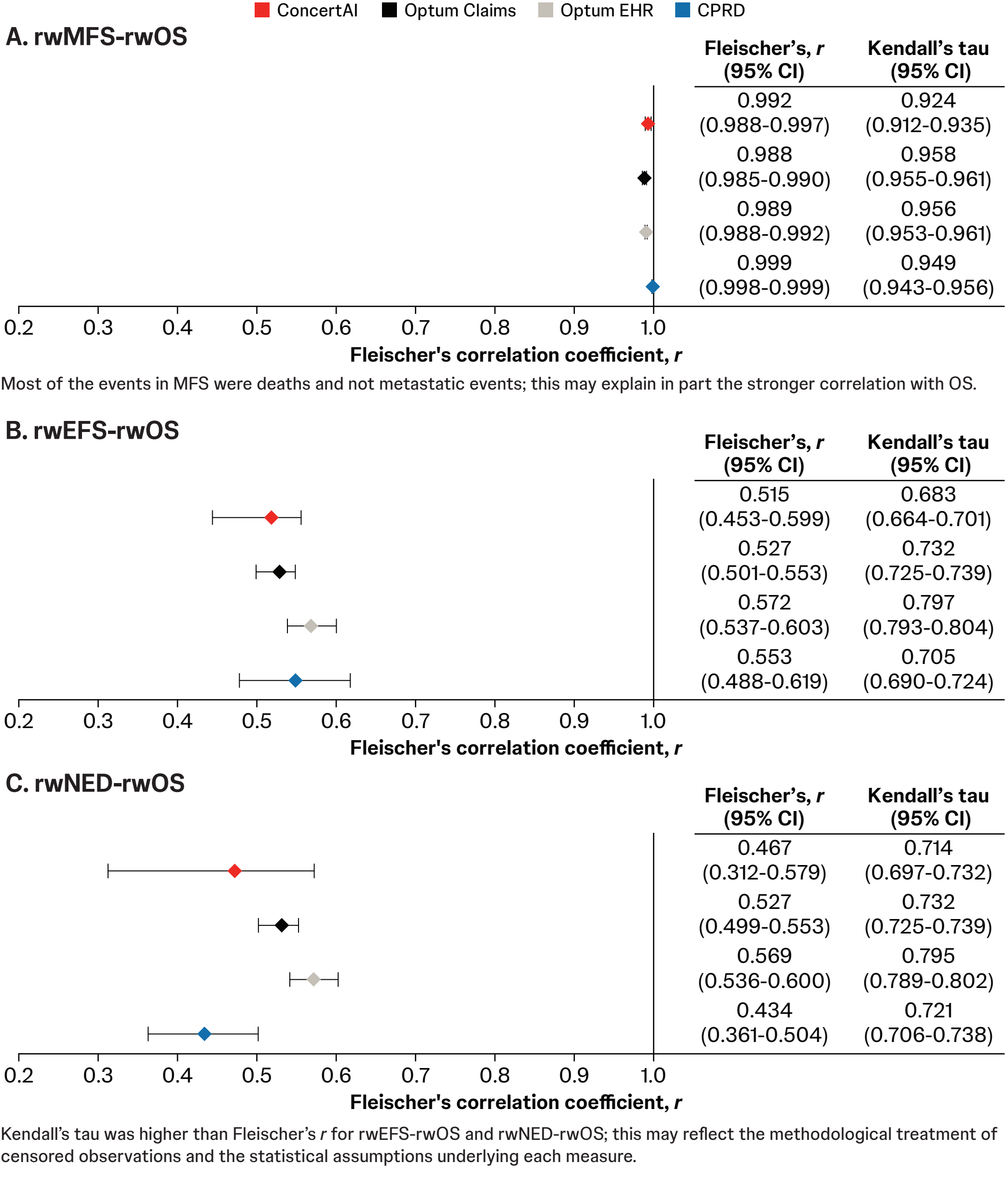
Figure 1: Correlation coefficients were strong between rwMFS and rwOS (A) and moderate between rwEFS and rwOS (B) and rwNED and rwOS (C)
