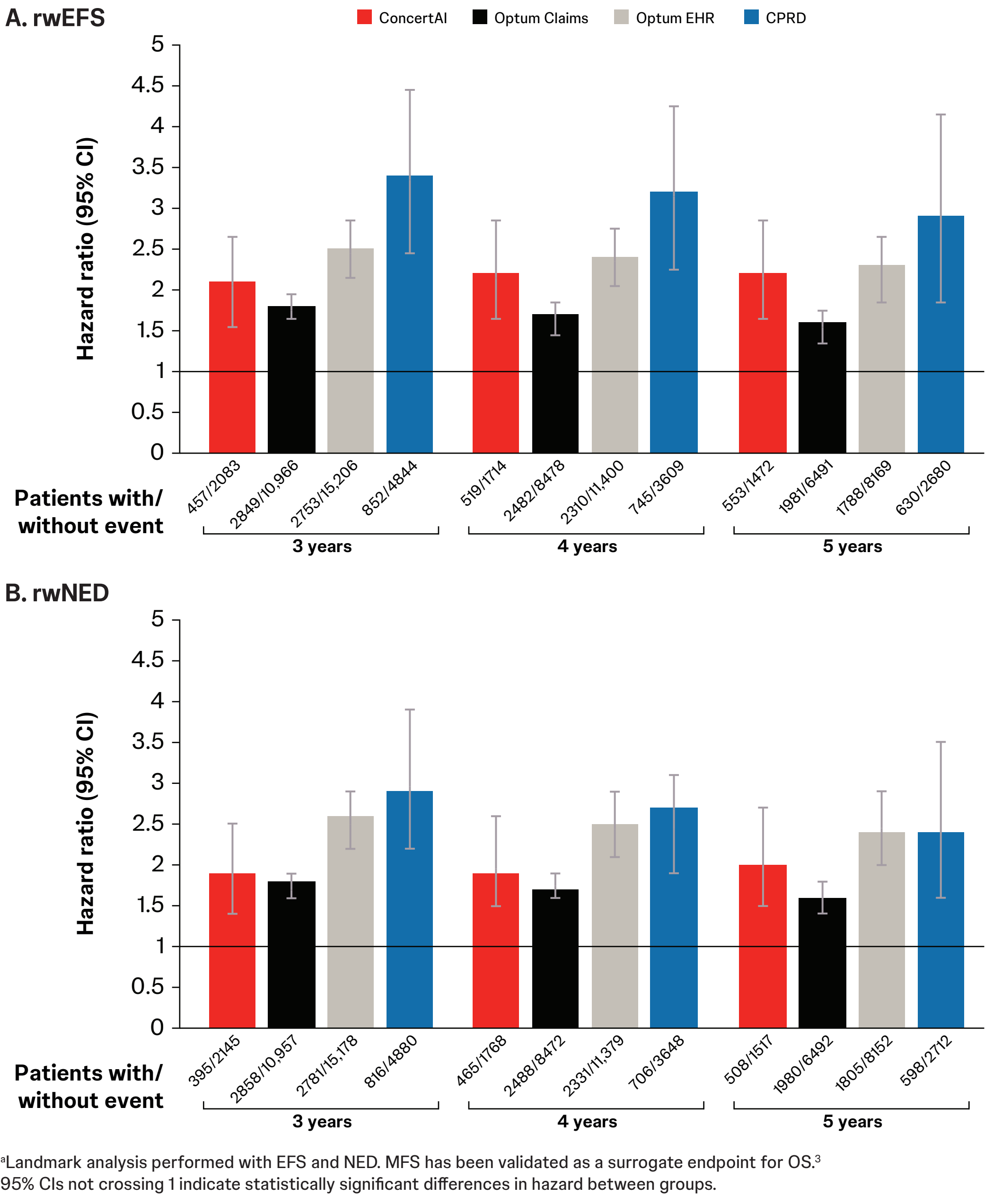
Figure 2: Landmark analyses of rwOS according to ICE landmark-event status (rwEFS and rwNED) a
